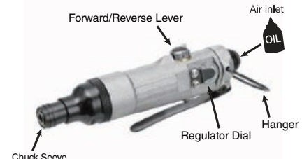
Forward/Reverse Lever
